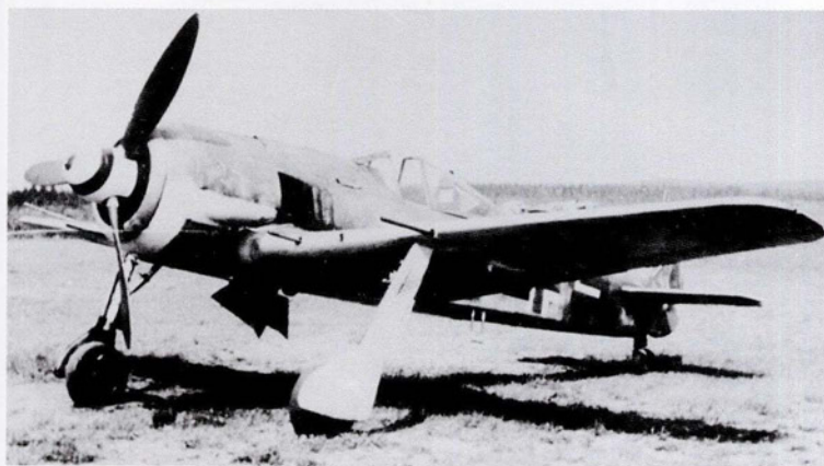
ABOVE, ABOVE RIGHT AND RIGHT: Another aircraft of Gefechtsverband Kuhlmei was this Fw 190 A-6 'White 7', W.Nr. 531056, of 4./JG 54, photographed at Käkisalmi in early July. In addition to the overpainting of the yellow area at the base of the rudder and the lower part of the yellow fuselage band, some parts of the camouflage finish have also been resprayed, most noticeably on the fin and the area around the tactical number and II. Gruppe bar. The white outline swastika on the fin is unusual at this time of the war.
